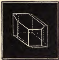
Crystal of Copper Sulphate.
